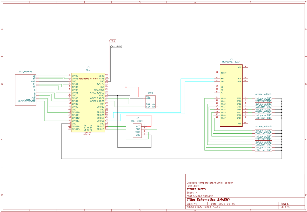
Figure 72: Electrical schematics
