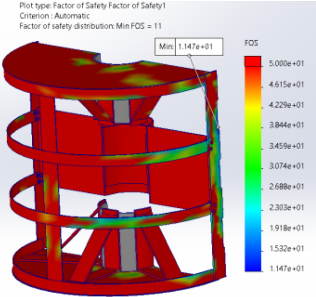
Figure 70: Factor of Safety
