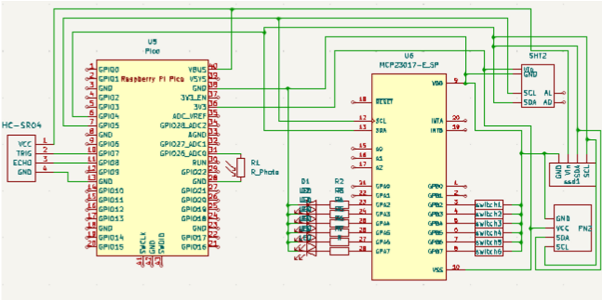
Figure 84: Schematic of prototype
