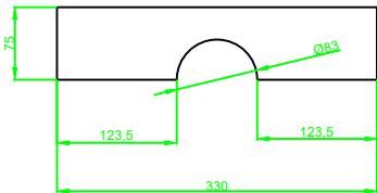
top and bottom piece back (2x)
