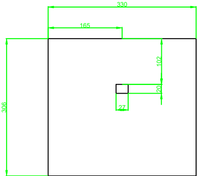
Back panel with cutout for screen
