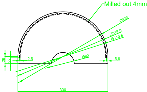
2 x end pieces round with milling to fit plexiglass
