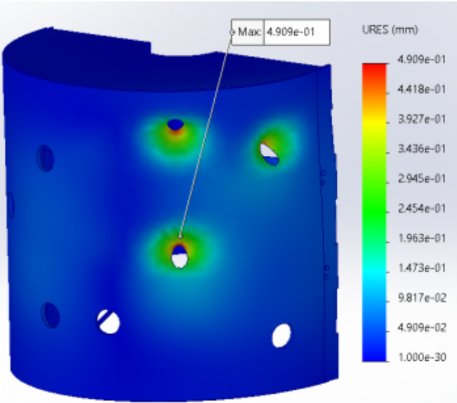
Figure 66: Simulated Displacement
