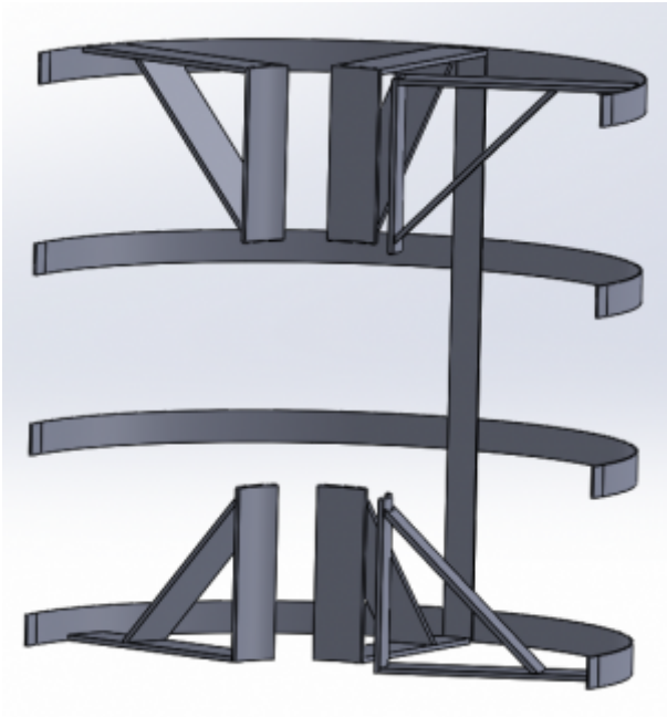
Figure 56: Supportive framework
