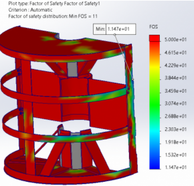
Figure 67: Factor of Safety
