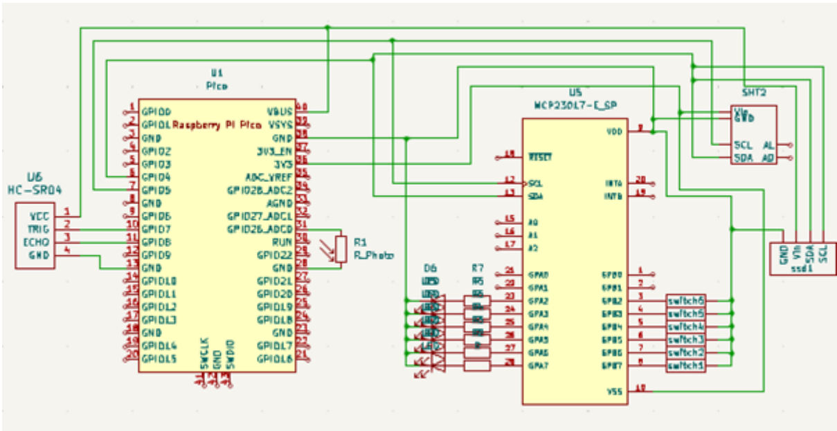
Figure 81: Schematic of prototype
