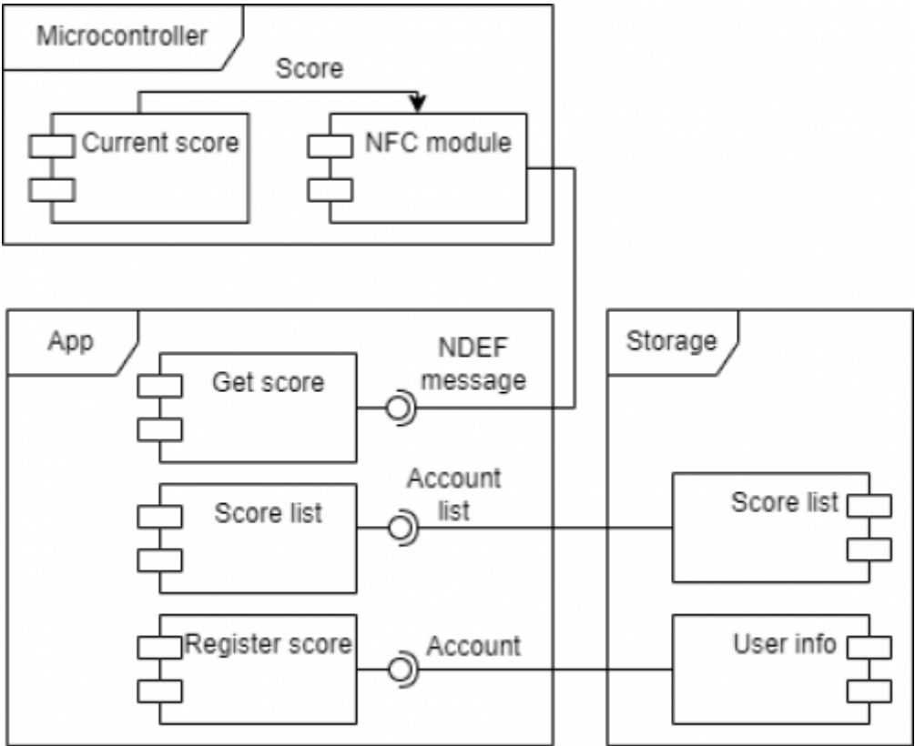
Figure 72: Component diagram of the system
