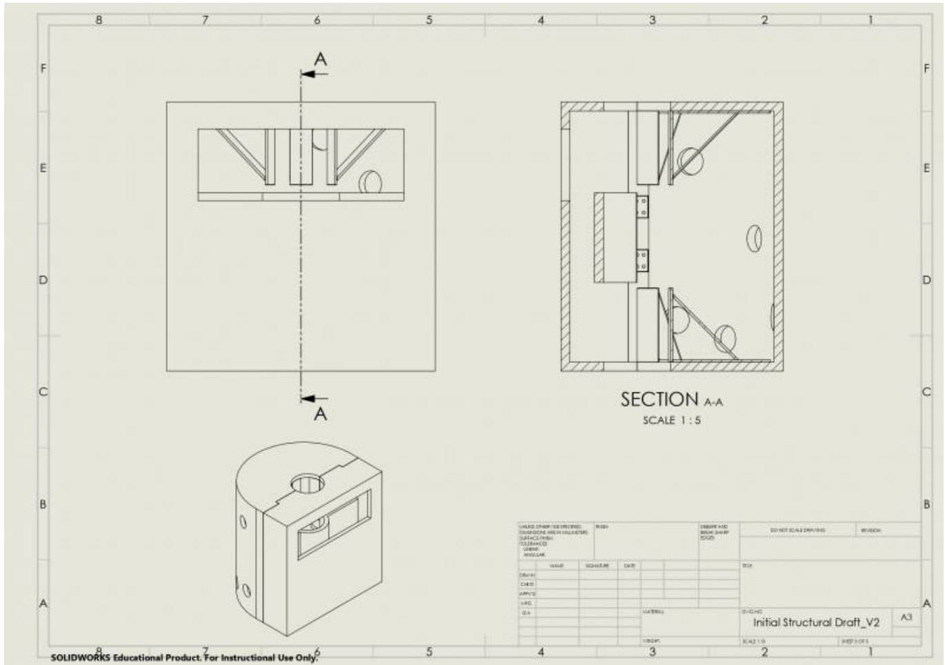
Figure 59: Initial structural drawings
